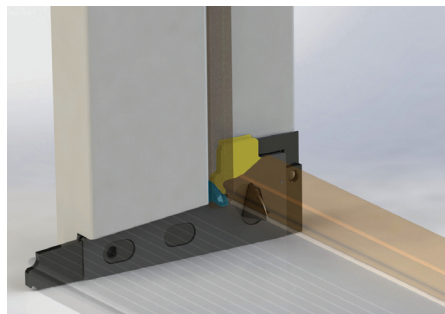
Works with no corner pad: Z-End Base™ provides protection against water infiltration.
