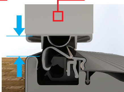
Loose margin: Sill cap rises to prevent leaks and drafts.
